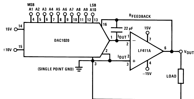
Figure 29. 10-Bit Linear DAC with No V_{OS} Adjust
